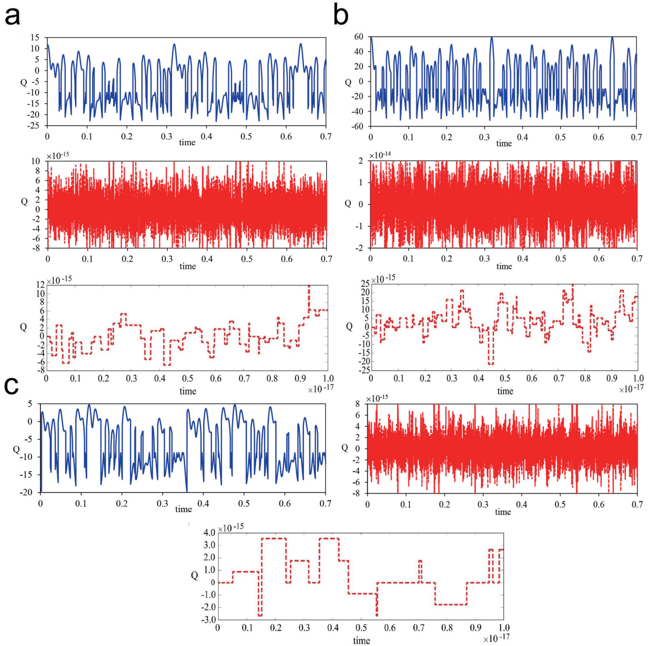
Fig. 5. The macro-quantum potential energy ( Q ) for (a) L=1 , x=0.1 , \gamma=1.0 (b) L=0.1 , x=0.01 , \gamma=0.01 . and (c) L=1.5 , x=0.5 , \gamma=2 . The real component is chaotic (non-periodic) and therefore non-coherent. The imaginary part is shown to fluctuate about zero and when 'zoomed-in' in time clearly reveals a unique informational pattern. Real component is shown as a continuous line (blue) and imaginary component is shown as a dashed line (red).
