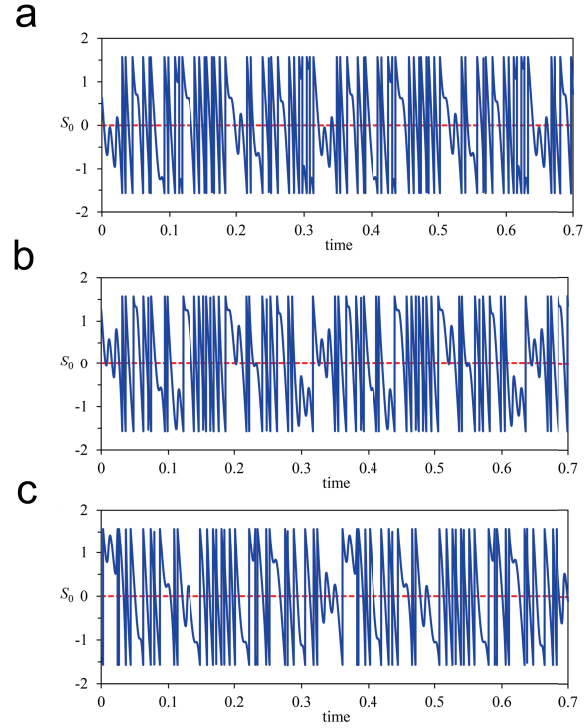
Fig. 2. Phase function ( S_0 ) versus time ( t ) for L=1 , \gamma = 1.0 , x=0.1 (Fig. 2a), L=0.1 , \gamma = 0.02 , x=0.01 (Fig. 2b) and L=1.5 , \gamma = 2 , x=0.5 (Fig. 2c). The phase synchrony of the dipole-bound electron oscillations is only in the real component of the phase function. Its amplitude varies between -\pi/2 and +\pi/2 showing coherence on phase (resonance). The imaginary component of the phase function remains close to zero. Real component is shown as a continuous line (blue) and imaginary component is shown as a dashed line (red).
