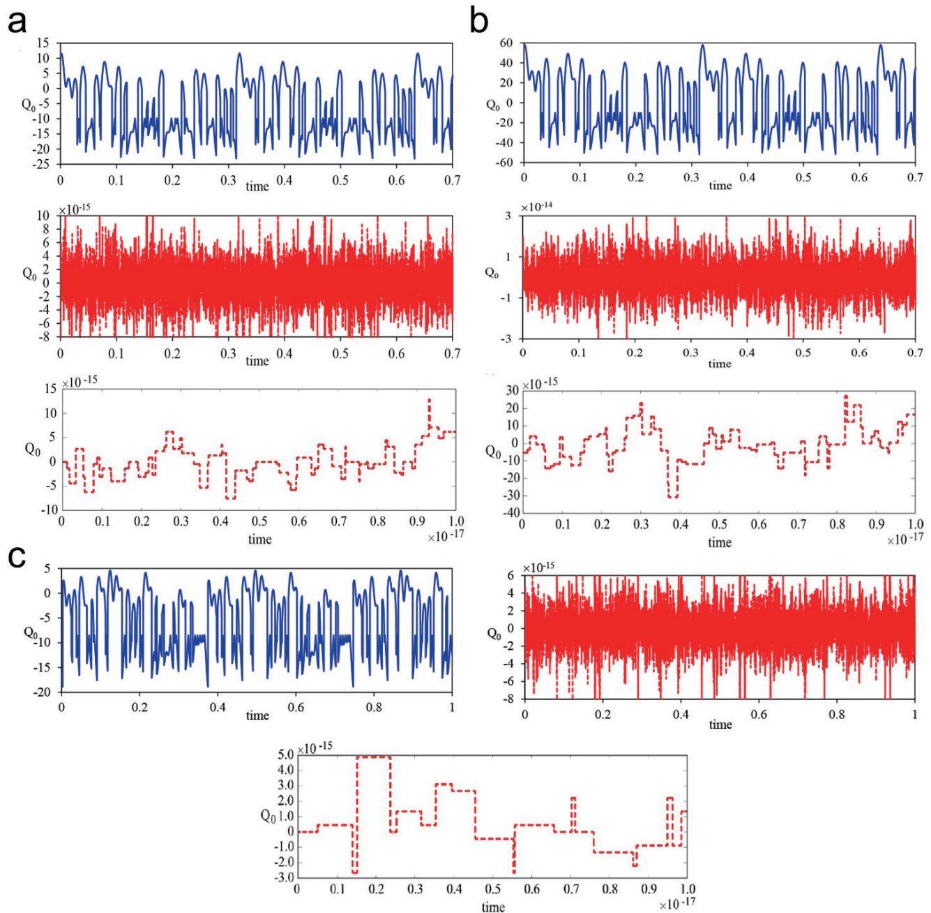
Fig. 4. The reduced macro-quantum potential energy ( Q_0 ) for (a) L=1 , x=0.1 , \gamma=1.0 (b) L=0.1 , x=0.01 , \gamma=0.01 . and (c) L=1.49 , x=0.5 , \gamma=1.9 . The real component is periodic and therefore coherent. The imaginary part is shown to fluctuate about zero and when 'zoomed-in' in time produces a unique informational pattern. Real component is shown as a continuous line (blue) and imaginary component is shown as a dashed line (red).
