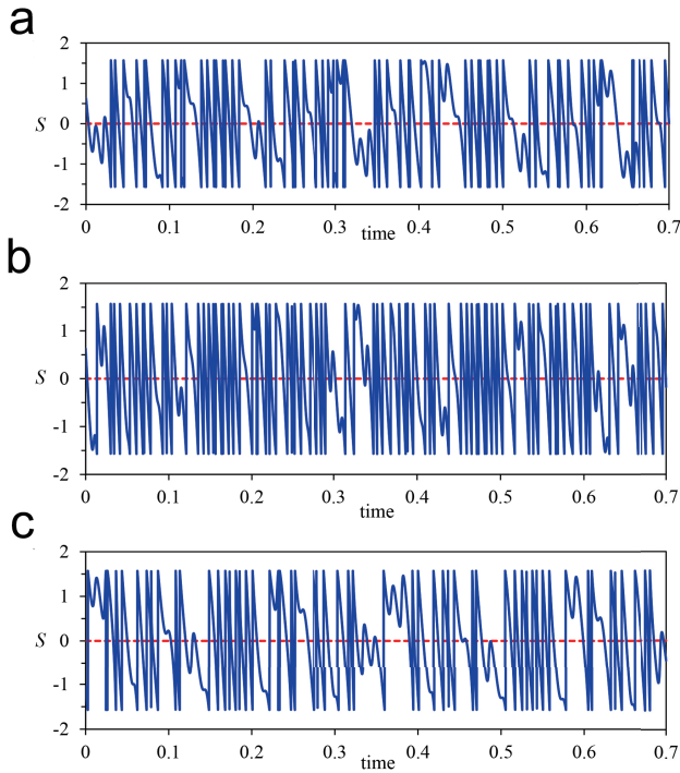
Fig. 3. Phase function ( S ) versus time ( t ) for L=1 , \gamma=1.0 , x=0.1 (Fig. 3a), L=0.1 , \gamma=0.01 , x=0.01 (Fig. 3b) and L=1.5 , \gamma=2 , x=0.5 (Fig. 3c) in the presence of classical potential energy U=1 . The phase differences of the dipole-bound electron oscillations are asynchronous as evident from the real component of the phase function. Its amplitude varies between -\pi/2 and +\pi/2 showing non-coherence. The imaginary component of the phase function remains close to zero. Real component is shown as a continuous line (blue) and imaginary component is shown as a dashed line (red).
